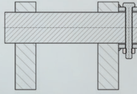
Traditional straight pin with locking ring
