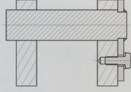
Traditional straight pin with flag washer
